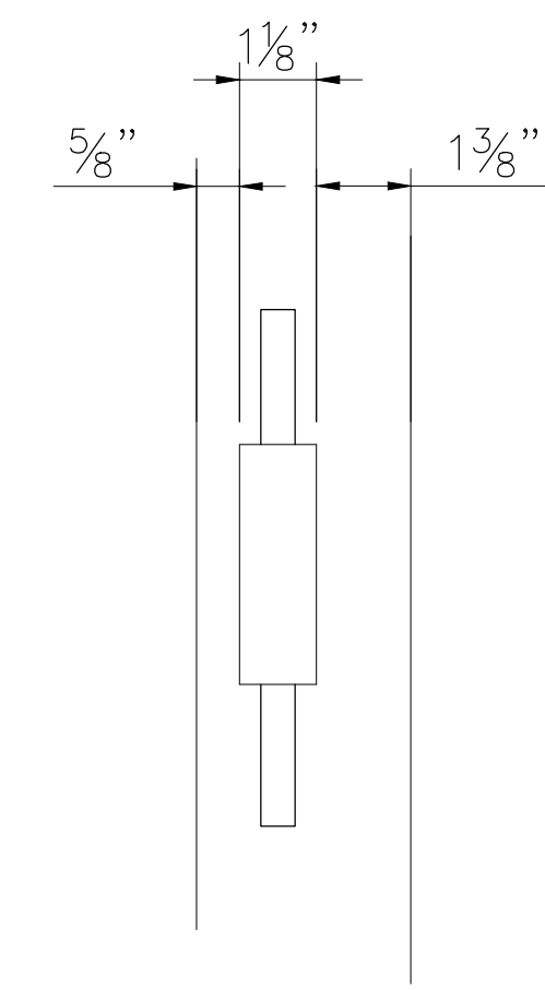
DETAIL "1"
